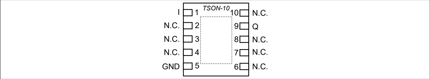
Figure 2 Pin configuration
